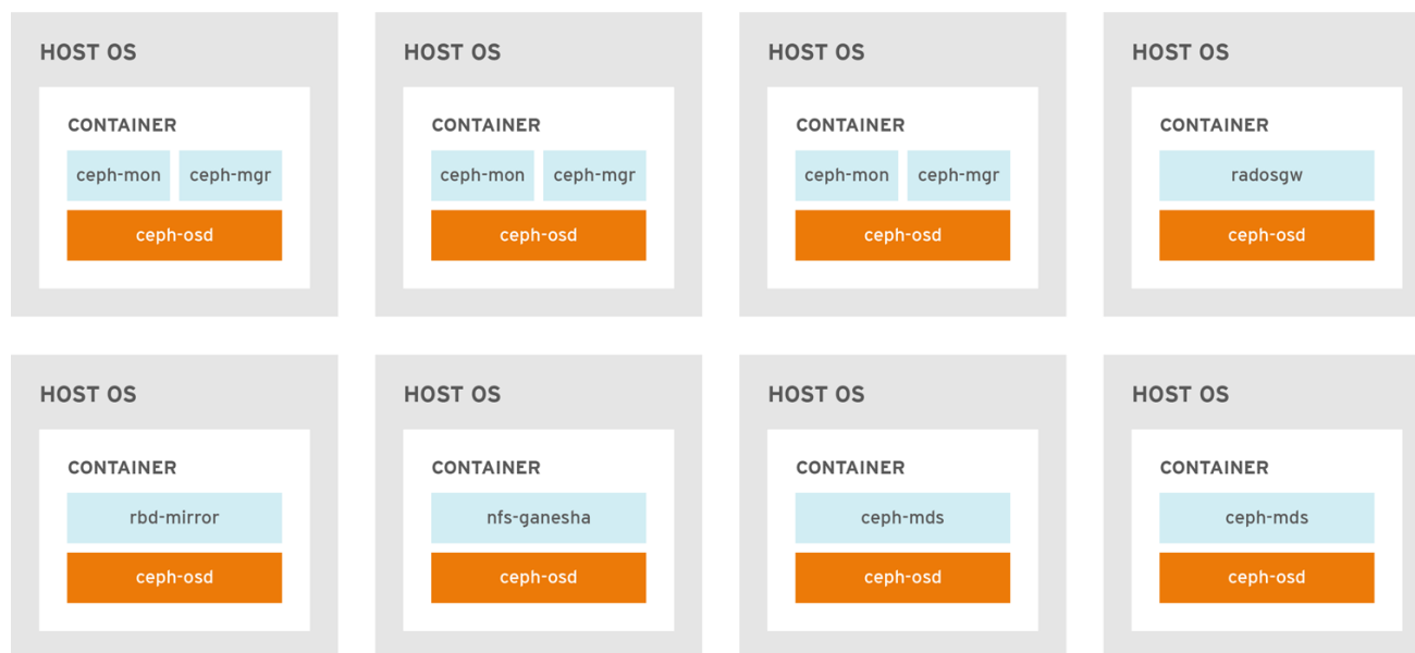
Figure 2.1. Colocated Daemons
