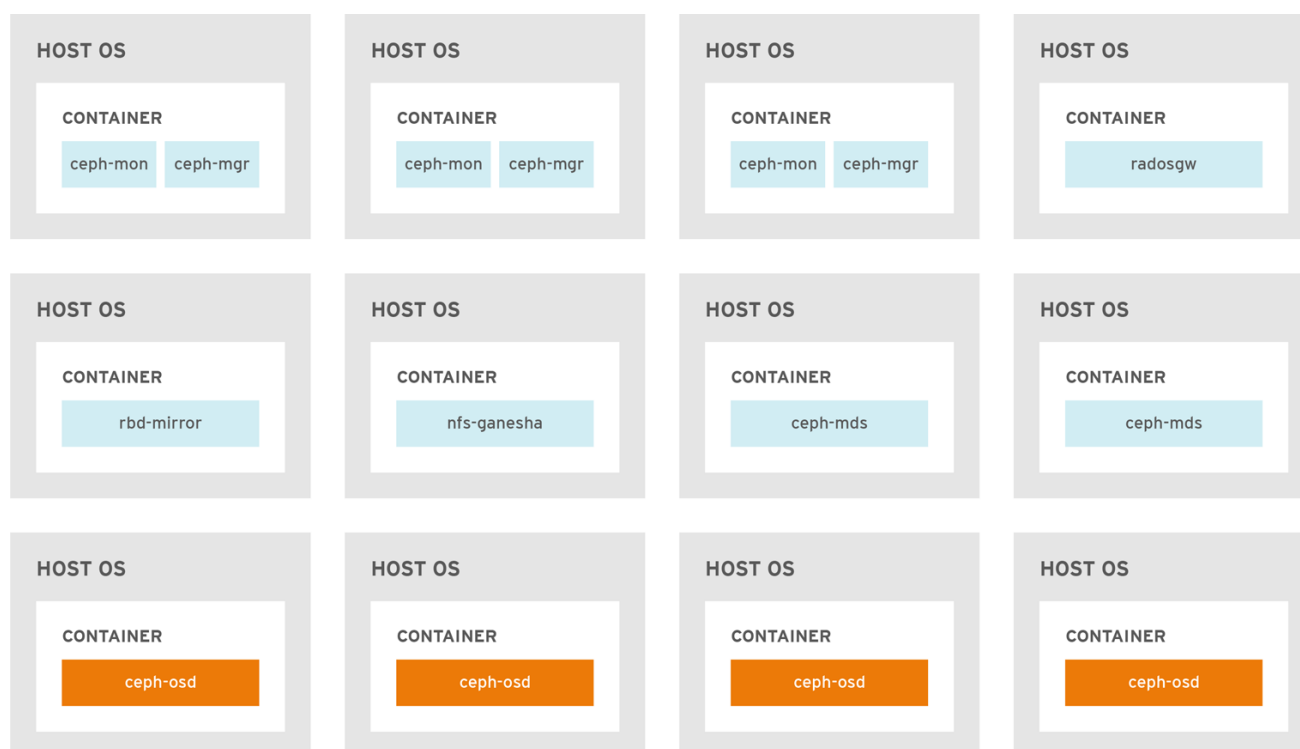
Figure 2.2. Non-colocated Daemons
